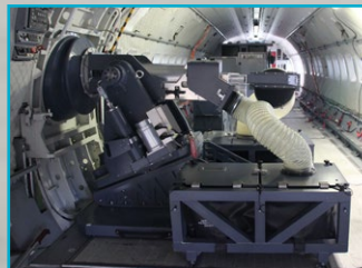
27 mm autocannon and Door Gun System (DGS)
