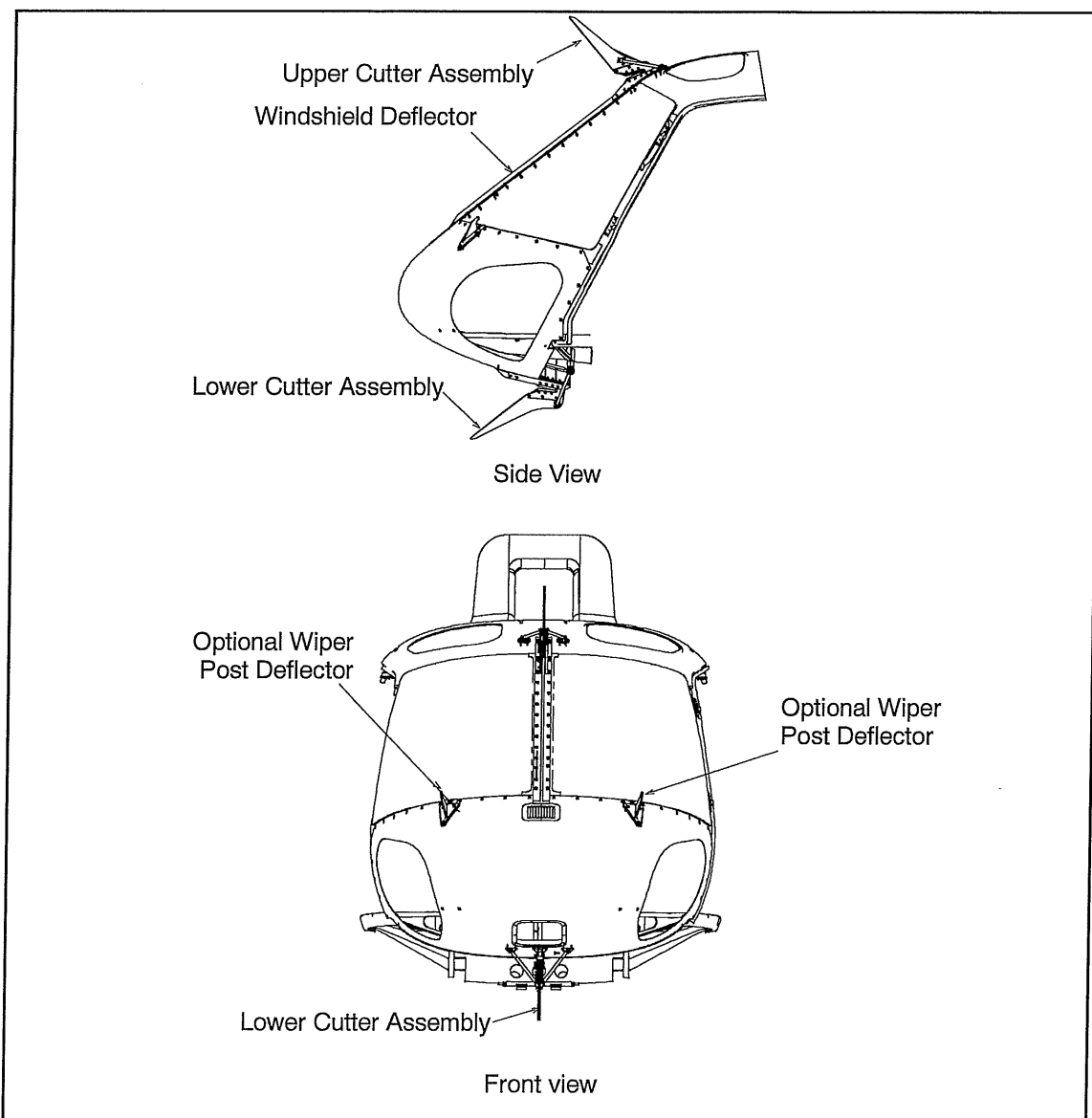
Figure 1 General Layout
