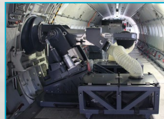
27 mm autocannon and Door Gun System (DGS)
