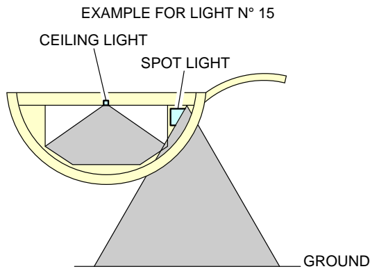
Exterior Lighting (Sheet 5 of 5) FIGURE-2-10-0-991-005-A01
