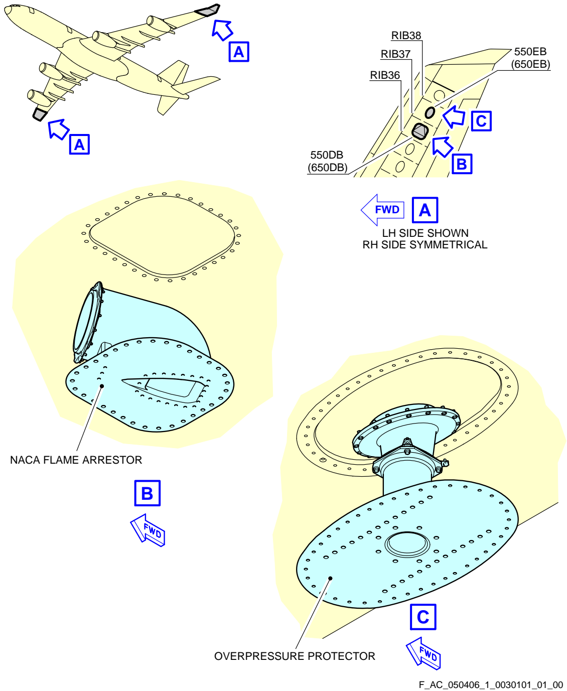
Ground Service Connections Overpressure Protector and NACA Flame Arrestor - Wing FIGURE-5-4-6-991-003-A01
