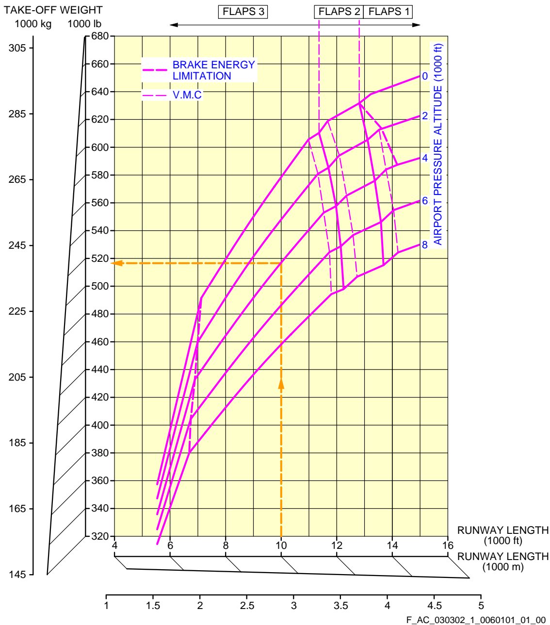
Take-Off Weight Limitation ISA +15°C (+59°F) Conditions – CFM56-5C3 engine FIGURE-3-3-2-991-006-A01
