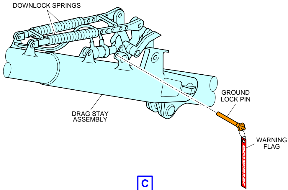
Centerline Landing Gear Safety Devices (Sheet 2 of 3) FIGURE-2-9-0-991-010-A01
