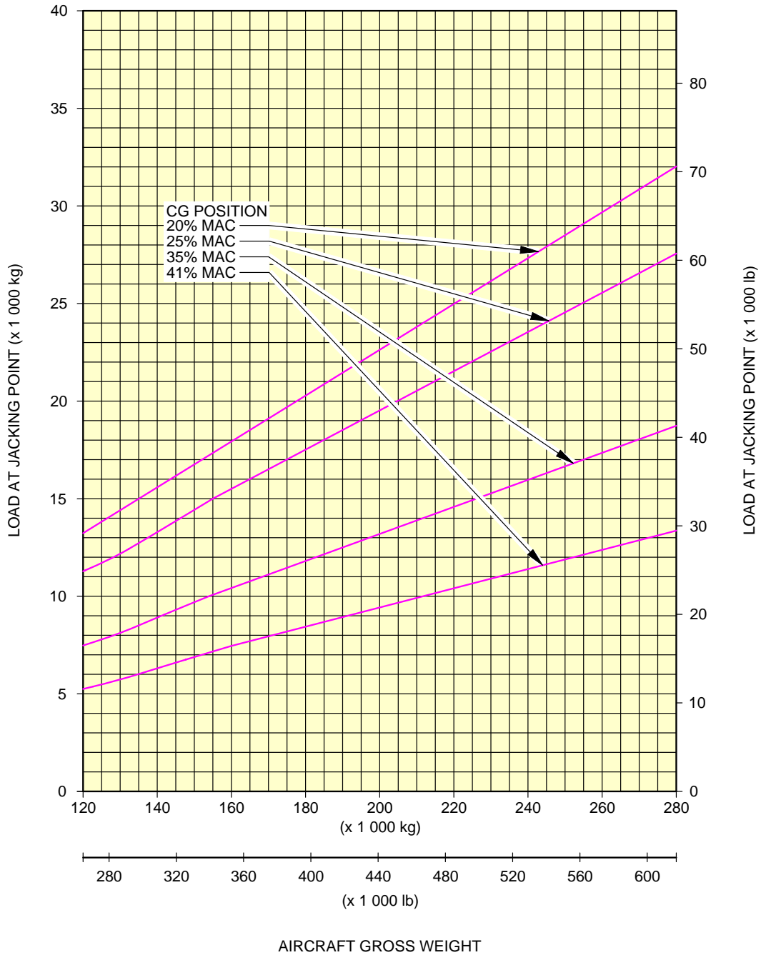
Jacking of the Landing Gear NLG Jacking Point Loads FIGURE-2-14-1-991-009-B01
