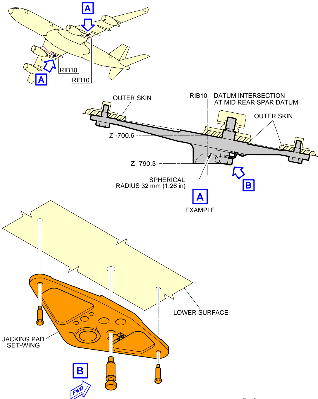
Jacking for Maintenance Wing Jacking Points FIGURE-2-14-0-991-010-A01
