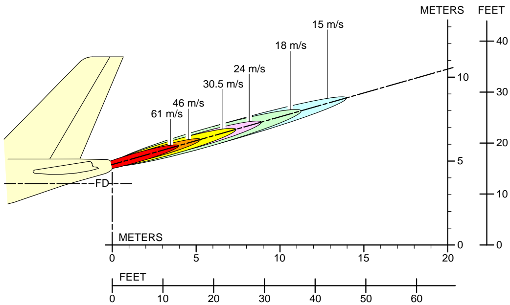
Exhaust Velocities and Temperatures GARRETT GTCP 331-350 FIGURE-6-4-1-991-002-A01
