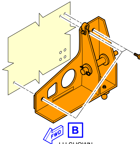
Support of Aircraft Location of Auxiliary Jacking Points (Sheet 2 of 2) FIGURE-2-14-2-991-002-B01
