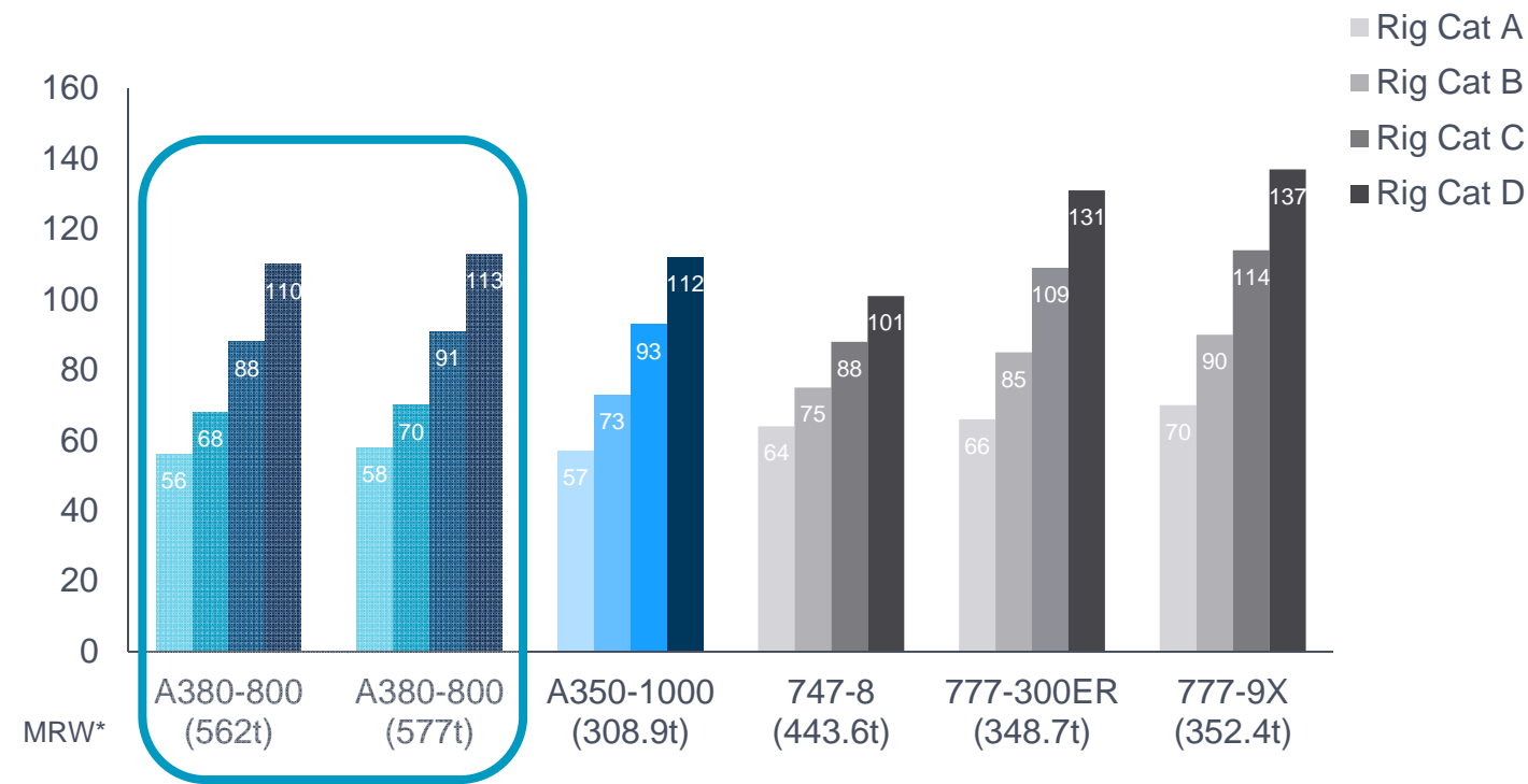
Aircraft Classification Number (ACN) – Rigid Pavement
