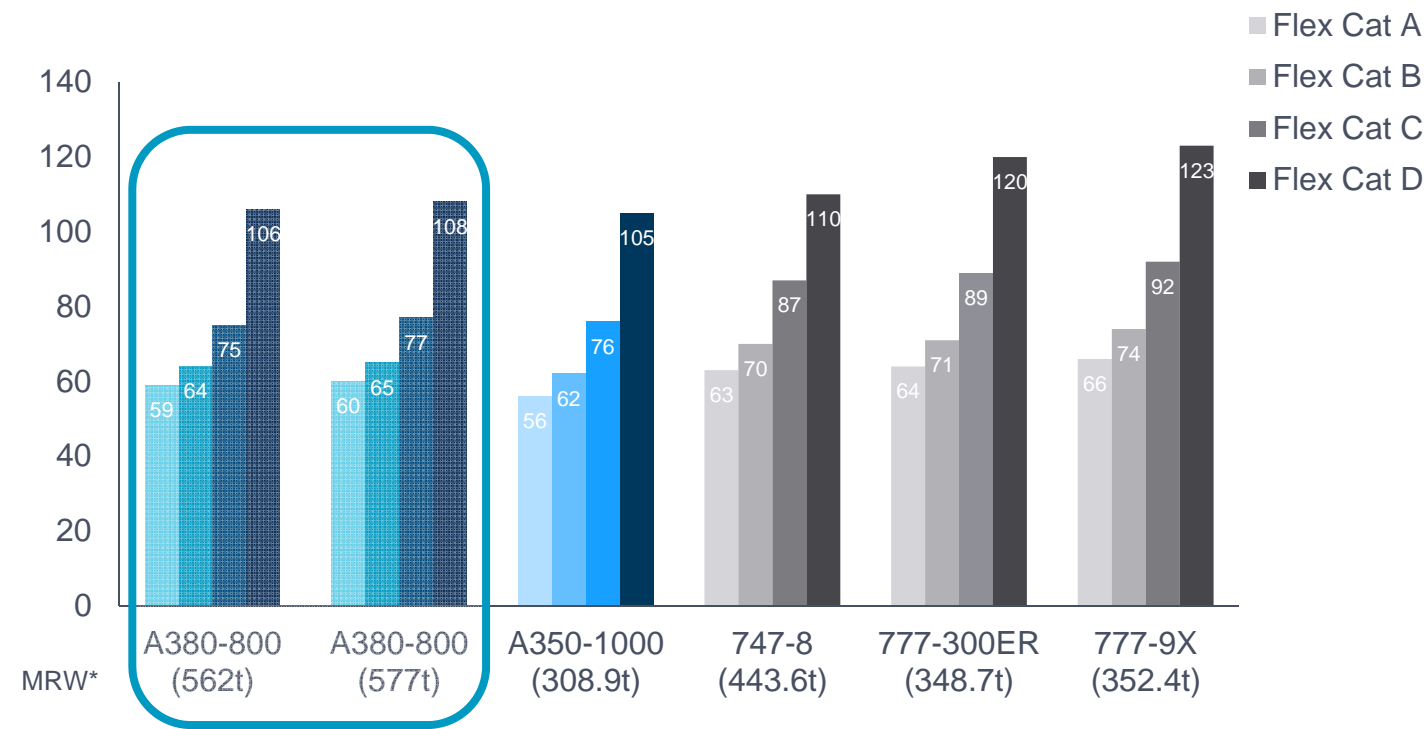
Aircraft Classification Number (ACN) – Flexible Pavement
